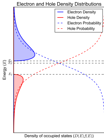
Figure: Left: Carriers density of a n-type semiconductor (Python-Simulated). Right: Schottky barrier of Metal-Semiconductor contacts (Source: Wikipedia )
