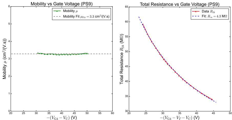
Figure: Extraction of \mu and R_{\infty} of PS9.
