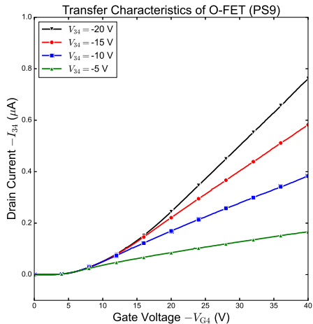
Figure: I-V Characteristics of Sample PS9.
