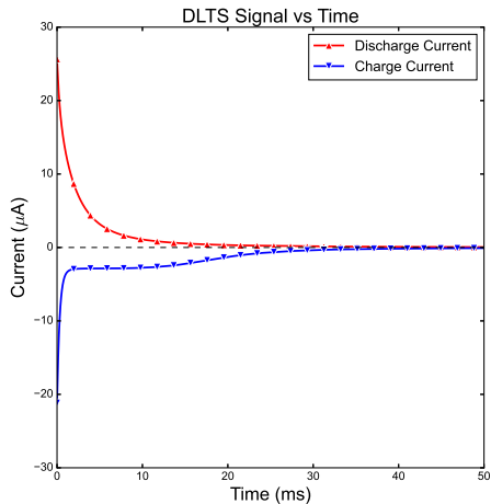
Figure: DLTS analysis for PS9.
